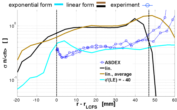
FIGURE 5. Time-averaged radial profiles of relative plasma density fluctuations. Again, the solid lines represent ESEL data, with the lowest lying, blue line for exponential form of the sheath dissipation term.
