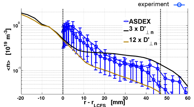
FIGURE 8. Time-averaged radial profiles of plasma density. Two solid lines represent ESEL simulations with theoretical value of the diffusion coefficient for particles multiplied by two different factors.
