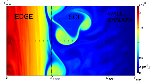
FIGURE 3. 2D computational domain of ESEL. The black dots represent the location of the numerical probes. The vertical axis represents the poloidal direction and the horizontal axis represents the radial direction. The colour code represents the plasma density. The SOL region width was around 27 mm for ASDEX Upgrade and around 37 mm for COMPASS.
