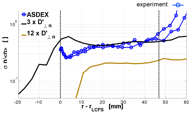
FIGURE 9. Time-averaged radial profiles of relative plasma density fluctuations. The solid lines represent ESEL data with theoretical value of the diffusion coefficient multiplied by a factor of 3 and 12.
