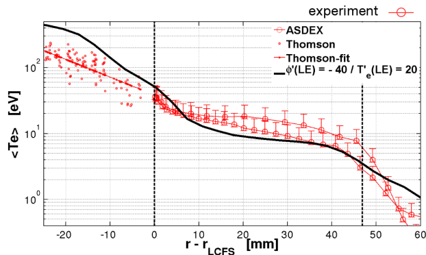
FIGURE 7. Time-averaged radial profiles of electron temperature (solid line - model, circles - experimental data). The experimental data consist from probe data (right of the LCFS line) and Thomson scattering data (left of the LCFS line - confined plasma).
