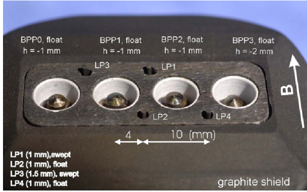
FIGURE 1. A photograph of the probe head with 4 Langmuir probes (LPs) and 4 ball-pen probes (BPPs) used in the ASDEX Upgrade. The vertical axis of the image corresponds to the direction parallel to \mathbf{B} and the horizontal axis corresponds to the poloidal direction in the tokamak [16].
