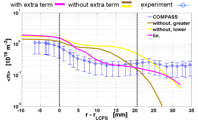
FIGURE 6. Time-averaged radial profiles of plasma density. The solid lines represent the ESEL data. Sheath dissipation term was used in the simulation represented by the pink solid line.
