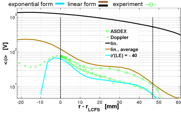
FIGURE 4. Time-averaged radial profiles of plasma potential. The solid lines represent ESEL data. In the simulation with the exponential form of the \Psi (blue line) the value of electric potential on LE of the computational domain was set as \phi'(LE) = -40 .
