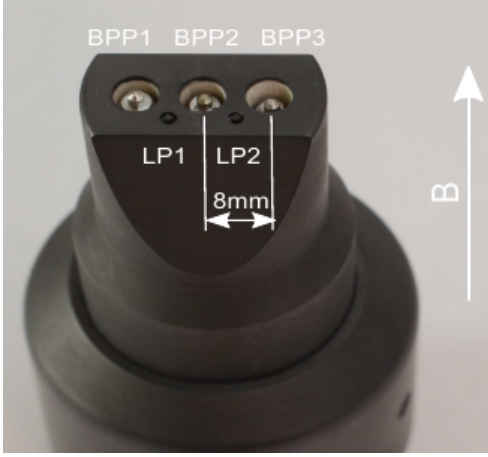
FIGURE 2. Photograph of the COMPASS probe head with 2 Langmuir probes (LPs) and 3 ball-pen probes (BPPs). The vertical and horizontal direction of the image parallel to the probe head surface corresponds to the toroidal and poloidal direction respectively [18].
