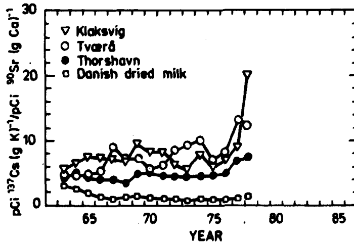
Fig. 2.3.3. \frac{M.U.}{B.U.} ratios in Faroese and Danish milk, 1963-1978.
