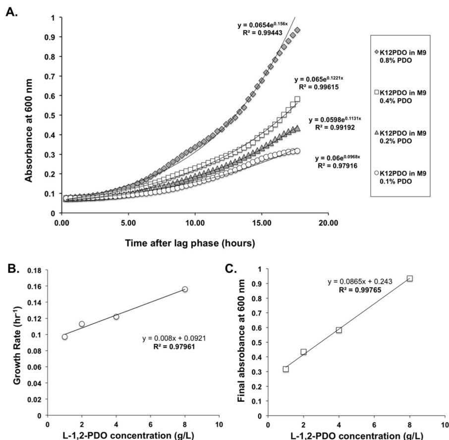
Fig. 2. Substrate concentration-dependent growth of K12PDO at different L-1,2-PDO concentrations.
