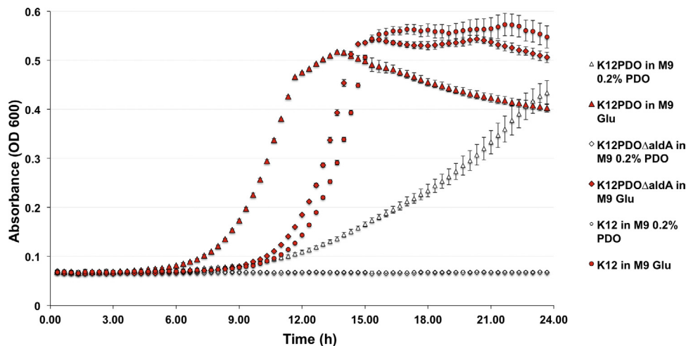
Fig. 3. Loss of function analysis of aldA .
