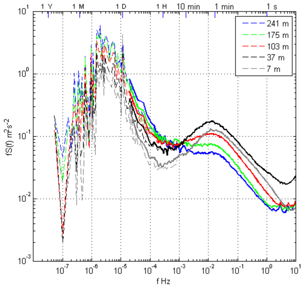
Figure 2. Spectra of wind speed at 5 heights at Østerild, from 1 year 10-min sonic data time series (dashed curves) and from day-long 20 Hz sonic time series (solid curves). Note 7 m is most likely sheltered by a surrounding forest.
