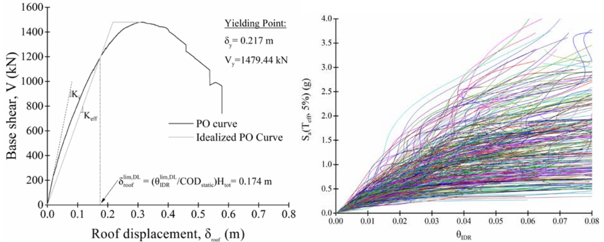
Figure 3. Pushover curve along with its bilinear idealization (left) and 300 IDA curves (right) for the initial code-compatible design of the 8-story RC building.
