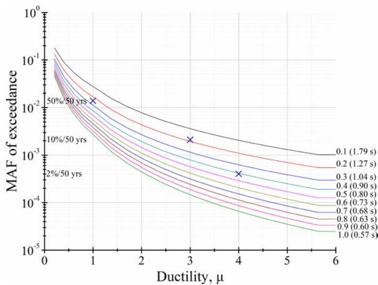
Figure 1. YFS contours at C_y = 0.10, \dots, 1.0 determined for an elastoplastic system ( \delta_y = 0.08 m) for a Californian site. The “x” symbols indicate three performance objectives, \mu = 1, 3, 4 at 50%, 10% and 2% in 50 yrs exceedance rates, respectively. The third objective governs with C_y \approx 0.408 and the corresponding period is T = 0.888 s.
