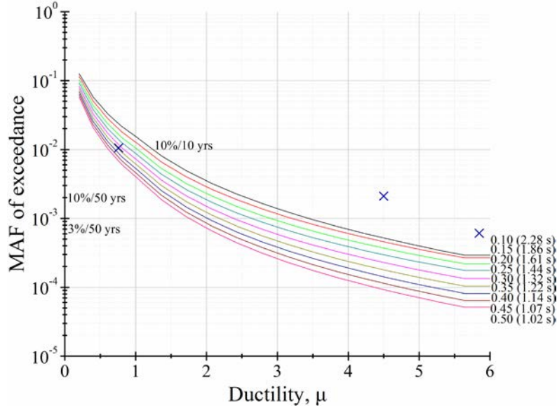
Figure 7. YFS contours at C_y=0.10, 0.15, \dots, 0.50 for designing the 8-story, RC space frame system, subjected to the adopted seismic hazard. “x” symbols represent the POs considered herein ( \mu=0.759, 4.5, 5.8 at 10% in 10yrs as well as 10% and 3% in 50 yrs exceedance rates, respectively). The DL objective (10% /10 yrs) governs with C_y \approx 0.336 and the corresponding period is T \approx 1.243 s.
