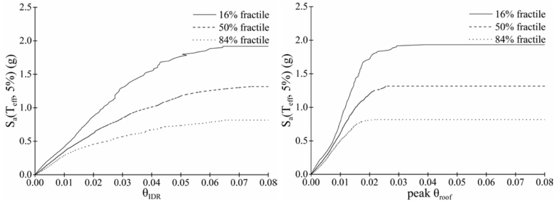
Figure 9. Summary (16%, 50% and 84% fractiles) of the IDA curves for the YFS-based, redesigned 8-story, RC space frame system: S_a(T_{eff}) vs \theta_{IDR} (left) and \theta_{roof} (right).
