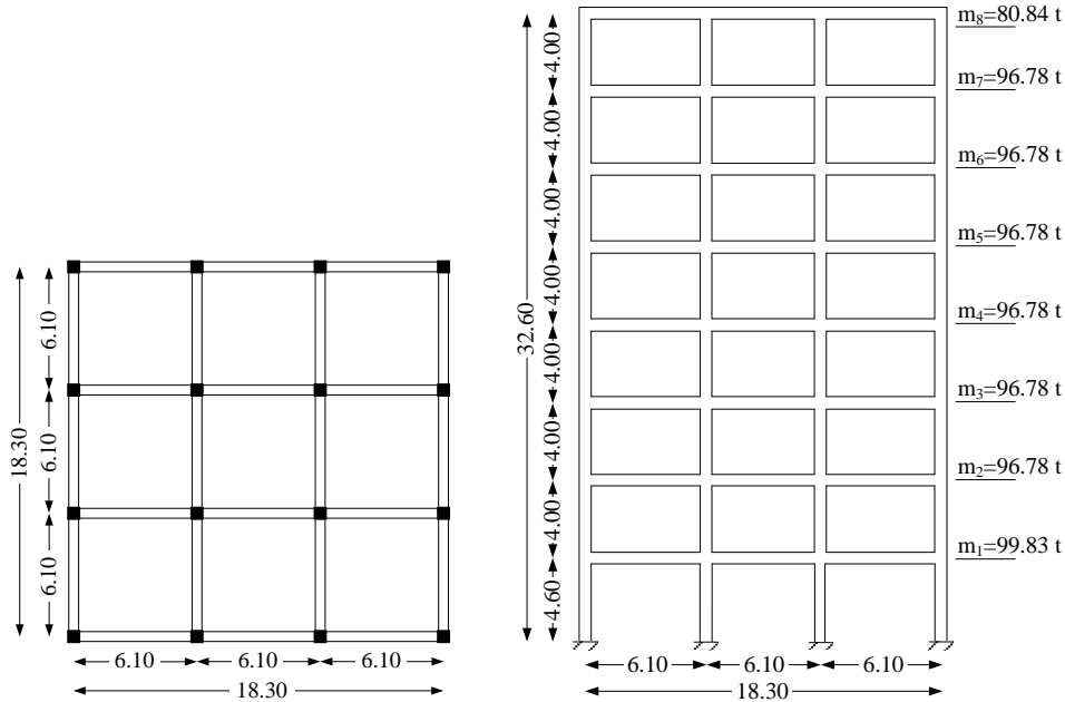
Figure 2. Plan view of a typical story (left) and internal frame (right) of the 8-story RC building studied herein.
