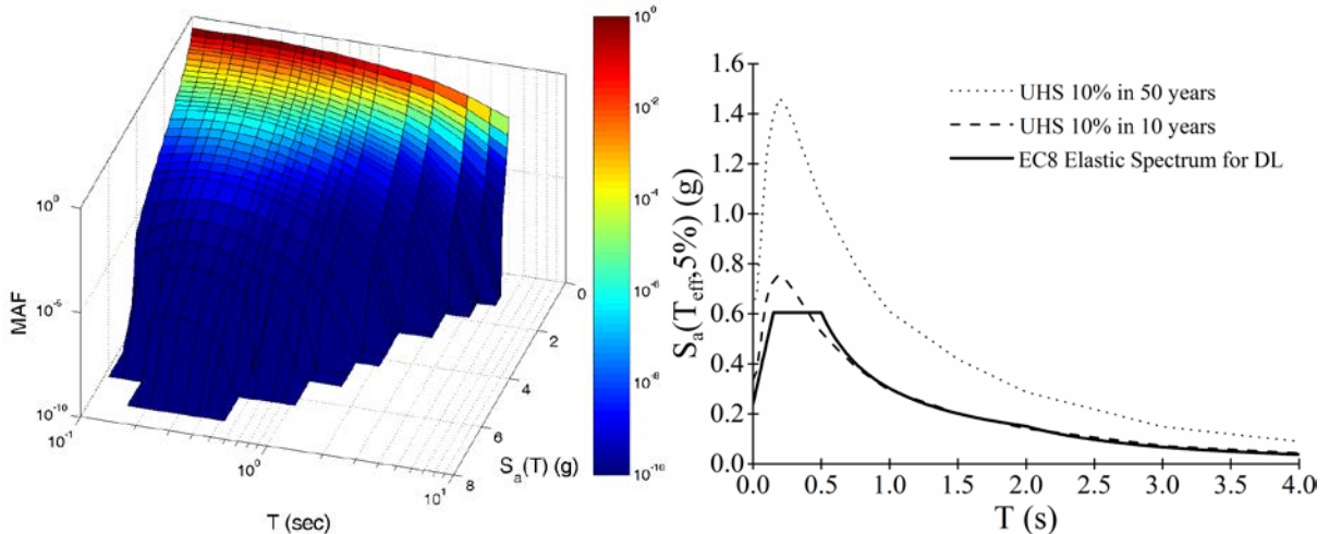
Figure 5. S_a hazard for the site: 3D plot of spectral acceleration hazard surface (left) and corresponding uniform hazard spectra plotted against the EN1998-1 elastic design spectrum appropriately reduced for DL checking (right).
