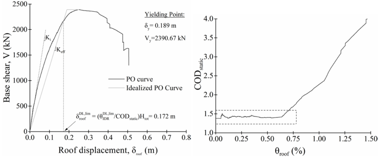
Figure 8. Pushover analysis of the YFS-based, redesigned 8-story, RC space frame system: Capacity curve and its bilinear idealization (left), COD calculation (right).
