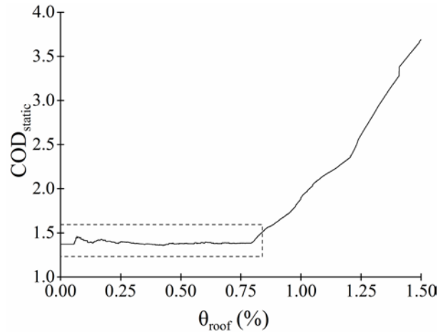
Figure 6. Coefficient of distortion ( COD ) calculation based on the pushover analysis for the initial code-compatible design of the 8-story RC building.
