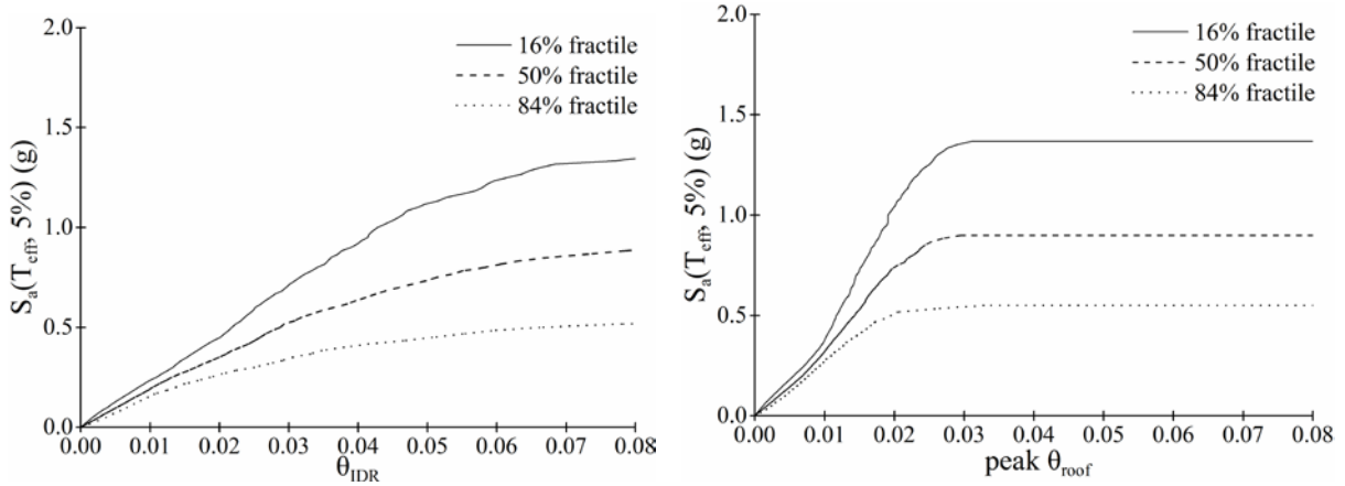
Figure 4. Summary (16%, 50% and 84% fractiles) of the IDA curves for the code-compatible designed 8-story, RC space frame system: S_a(T_{eff}, 5\%) versus \theta_{IDR} (left), and \theta_{roof} (right).
