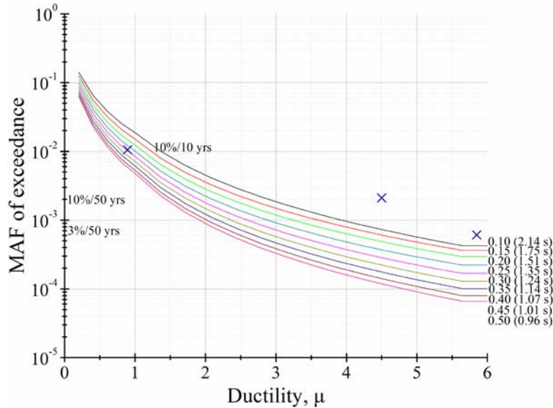
Figure 10. YFS contours at C_y=0.10, 0.15, \dots, 0.50 for designing the 8-story, RC space frame system, subjected to the adopted seismic hazard. “x” symbols represent the POs considered herein ( \mu=0.893, 4.5, 5.8 at 10% in 10yrs as well as 10% and 3% in 50 yrs exceedance rates, respectively). The DL objective (10% /10 yrs) governs with C_y \approx 0.293 and the corresponding period is T \approx 1.251 s.
