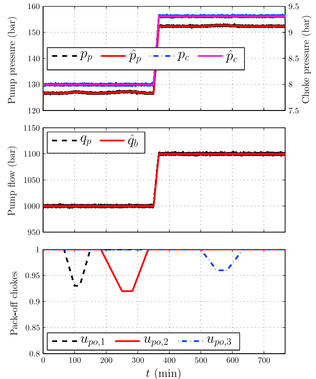
Fig. 3. Pressure and flow estimation, and valve openings simulating pack-offs.
