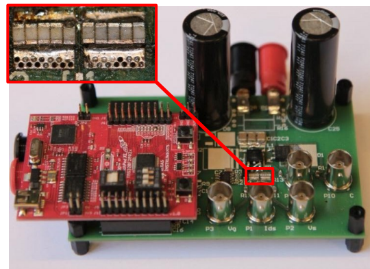
Figure 4. Double pulse tester prototype with integrated current shunt
