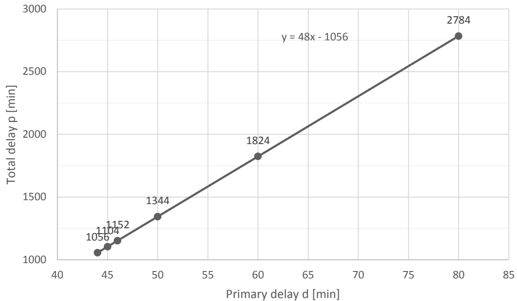
Figure 1 - Total delay measured on the line as a function of the primary delay given to the first train at the first station
