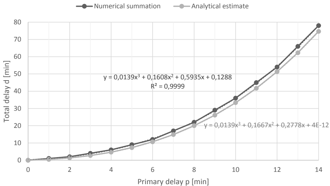
Figure 2 - Total delay measured as the numerical summation and estimated through the analytical formulation.
