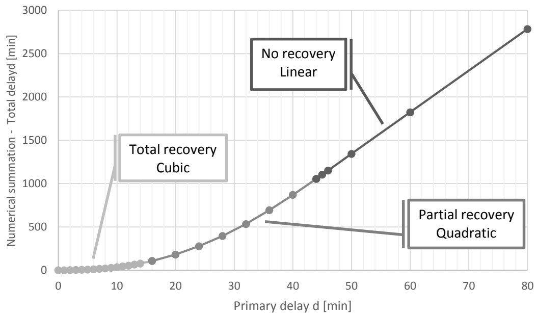
Figure 4 - Total delay summed in the numerical example.
