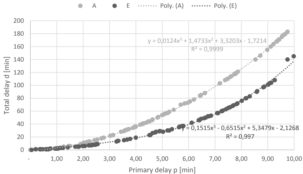
Figure 5 - Measured total delay on the suburban railway line Hellerup - Hillerød, as a function of the primary delay. Each curve represents the total delay generated delaying either railway line of the timetable.
