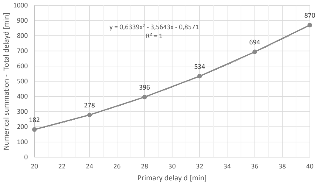
Figure 3 - The total delay numerically summed in the example. Partial recovery range.
