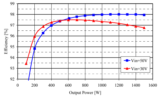
Fig. 7. Converter efficiency including drive power.
