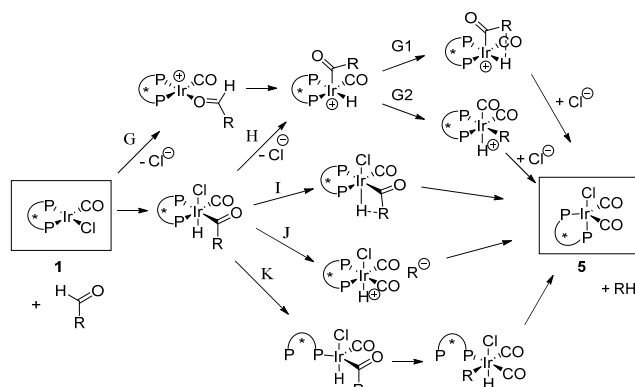
Scheme 6. Possible pathways for the decarbonylation of aldehydes. G) Substitution pathway. H) Oxidative addition followed by dissociation of chloride. I) A concerted migration pathway. J) R dissociates from the acyl complex. K) Phosphine dissociation pathway.
