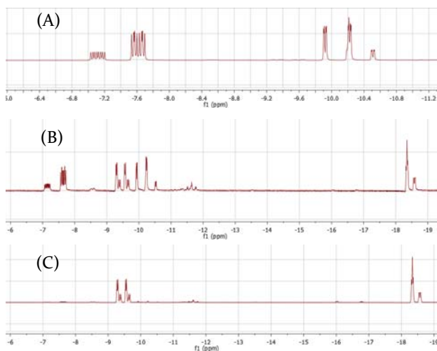
Figure 4. Hydride region in 1 H NMR spectra. (A) Spectrum recorded after 30 min where only hydrides from the kinetic isomers 2A and 2B are observed. (B) Spectrum recorded after removal of benzene, where an isomerization had started to occur. (C) Spectrum recorded after removal of toluene,
