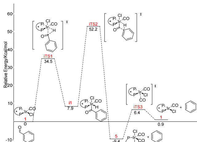
Figure 11. The lowest energy profile of the decarbonylation pathway I.
