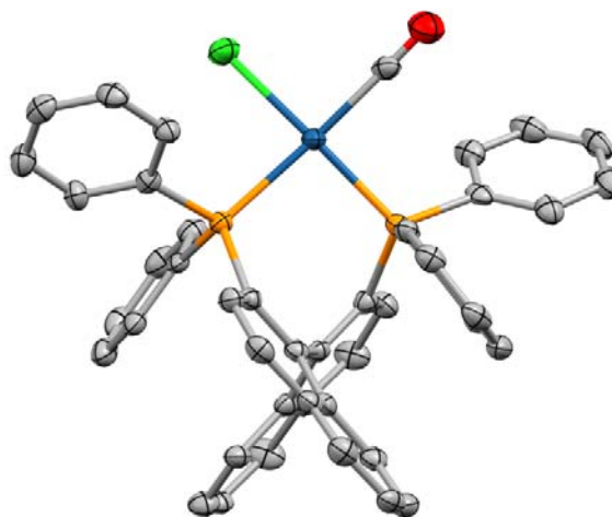
Figure 1. Crystal structure of IrCl(CO)(S)-BINAP.
