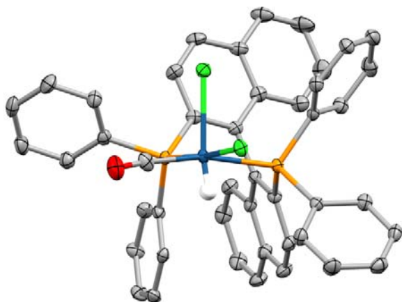
Figure 6. Crystal structure of \text{IrHCl}_2(\text{CO})(\text{R})\text{-BINAP} .
