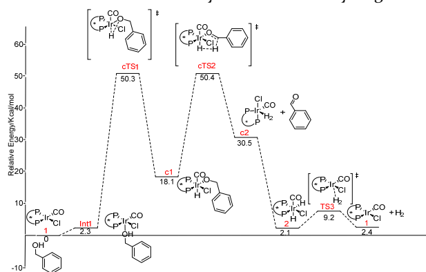
Figure 8. Energy profile for the dehydrogenation pathway C.
