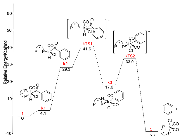
Figure 12. The lowest energy profile of the decarbonylation pathway K.
