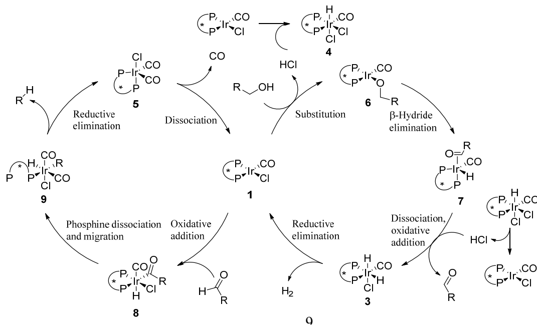
Figure 13. The proposed catalytic cycles.
