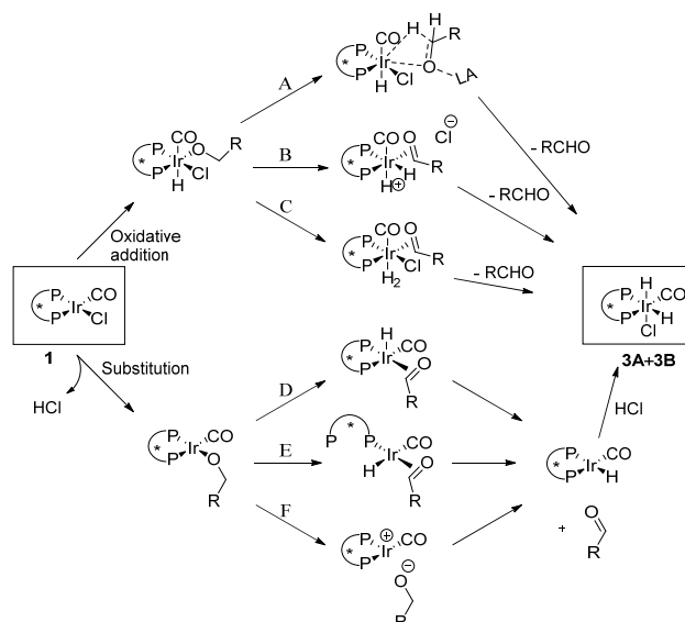
Scheme 2. Possible routes to formation of 3A and 3B . A) Pathway without a vacant site. B) Chloride dissociation followed by \beta -hydride elimination and ligand substitution. C) Hydride extracts the \alpha -proton forming a dihydrogen complex. D) Direct \beta -hydride elimination from the square planar iridium alkoxo complex. E) Phosphine dissociation prior to \beta -hydride elimination. F) Ionic pathway.
