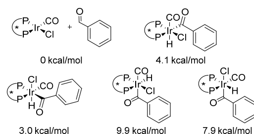
Figure 10. The four different geometrical isomers formed from oxidative addition of benzaldehyde.
