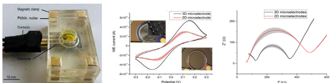
Figure 2 : (a) Experimental set-up, (b) and (c) Electrochemical characterisation (CV and EIS) of 3D and 2D chips (Data are presented as mean \pm standard deviation ( n = 3 ))
