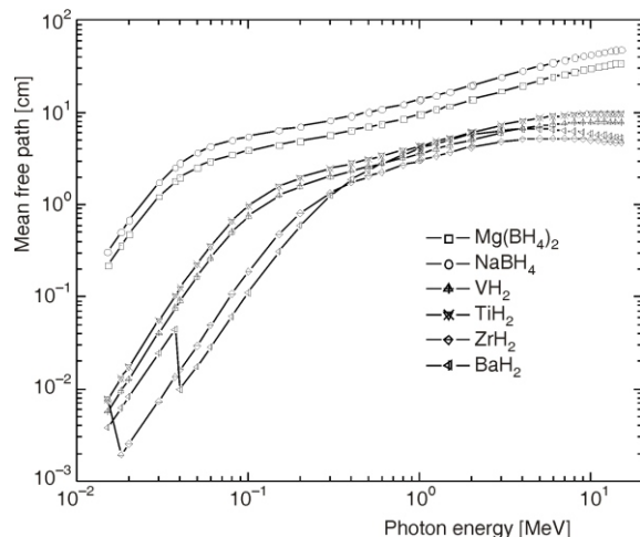
Figure 3. Mean free path in metal hydrides and borohydrides at photon energies 0.015-15 MeV
