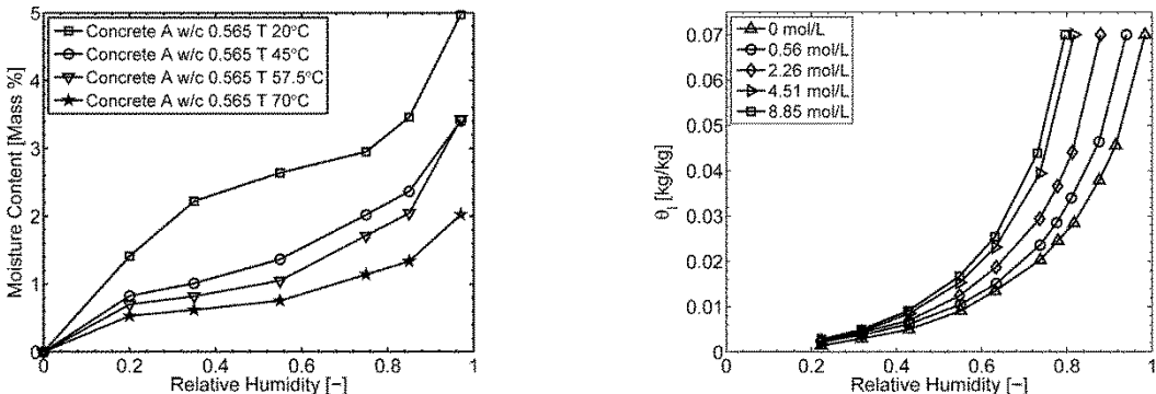
Fig. 3 Left: moisture storage for concrete at various temperatures (experimental data reproduced from Hundt & Kantelberg (1978)). Right: moisture storage of mortar specimens for varying sodium chloride concentrations (experimental data reproduced from Baroghel-Bouny & Wang (2011)).
