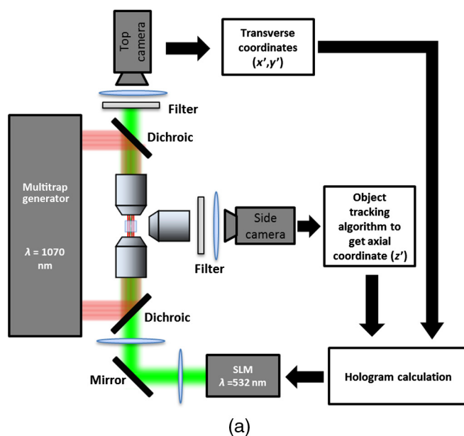
Fig. 2 (a) Schematic diagram of the biophotonics workstation for trapping and coupling experiments. (b) Graphical demonstration of diffractive coupling to a single microtool. The microtool is moved in three-dimensional (3-D) space using the counter-propagating trapping beams holding its spherical handles. The diffractive phase holograms are used to modulate each coupling beam to dynamically follow the position of the respective microtool in real time.
