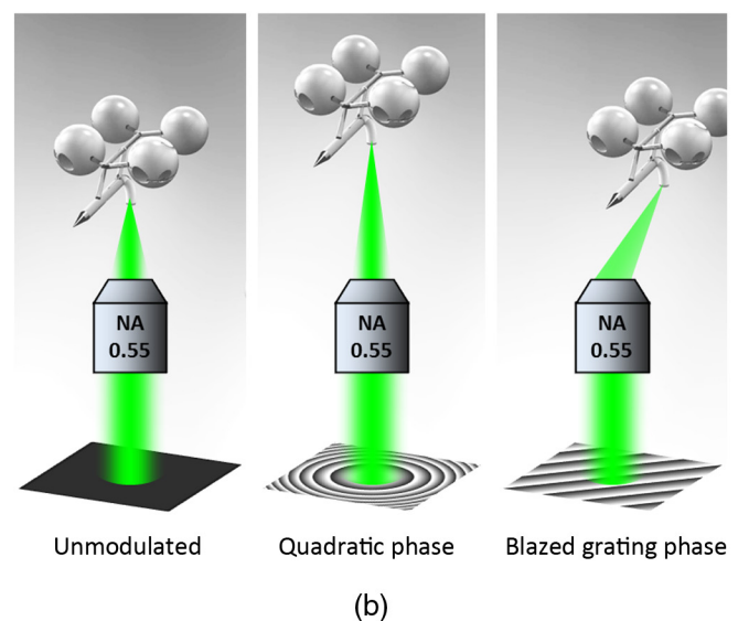
Fig. 2 (a) Schematic diagram of the biophotonics workstation for trapping and coupling experiments. (b) Graphical demonstration of diffractive coupling to a single microtool. The microtool is moved in three-dimensional (3-D) space using the counter-propagating trapping beams holding its spherical handles. The diffractive phase holograms are used to modulate each coupling beam to dynamically follow the position of the respective microtool in real time.
