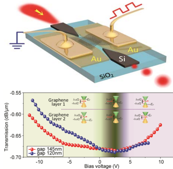
Figure 1. Upper: 3D schematic of the graphene plasmonic waveguide modulator. Down: Modulated transmission for 20 \mu\text{m} -long graphene plasmonic hybrid slot waveguides.
