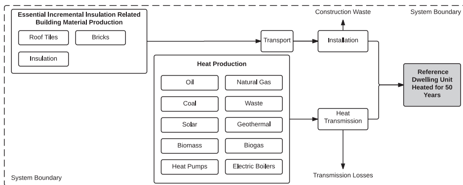
Fig. 2. System boundary and flows for LCA comparing IS2015 and IS2020
