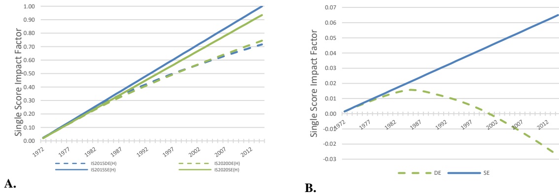
Fig. 3. Life Cycle Assessment with ReCiPe Hierarchist single score impact factor values based on internal normalization through division by maximum value. (A) Comparison of IS 2015 and 2020 Static and dynamic insulation scenarios total impact; (B) IS2020 static and dynamic energy scenario impact savings compared with IS2015, negative values indicate that IS2020 has a greater cumulative impact.
