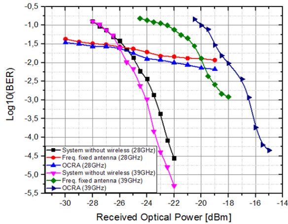
Fig.6. The performance analysis as a function of BER for 28 and 39 GHz frequency bands.
