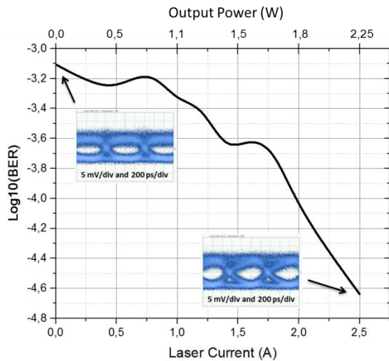
Fig. 7. Measured BER as function of the laser control current at 39GHz.
