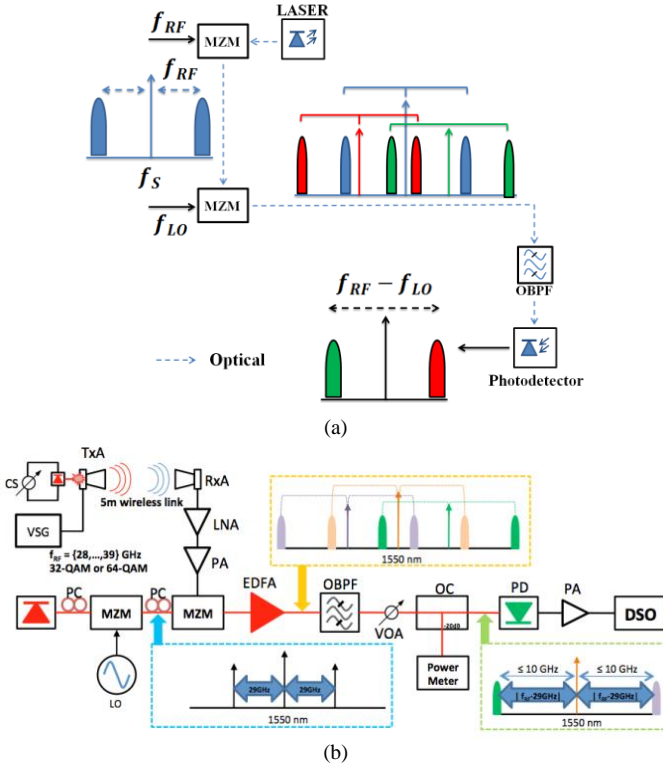
Fig. 2. The first approach for PDC: CS: current source, TxA: transmitting antenna, RxA: receiving antenna, PC: polarization controller, EDFA: erbium doped fiber amplifier, OBPF: optical band pass filter, VOA: variable optical attenuator, PD: photodetector, PA: power amplifier, DSO: digital storage oscilloscope. (a) Schematic. (b) Experimental setup.
