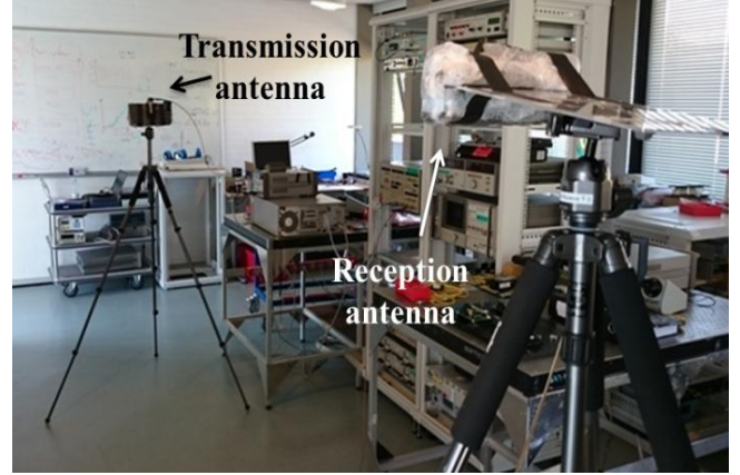
Fig. 5. Wireless setup used for the BER measurements.
