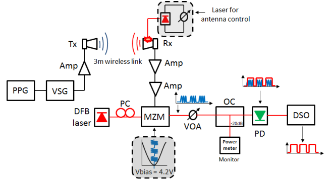
Fig. 3. Experimental setup of the second photonic downconversion approach, including the pulse pattern generator.
