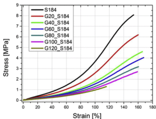
Fig. 10 Stress-strain behaviour of various compositions obtained from tensile measurements.
