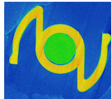
Fig. 4. Reconstruction slice, modified in Fiji image processing software, of the two-part component showing the complete absence of artefacts on the surfaces.
