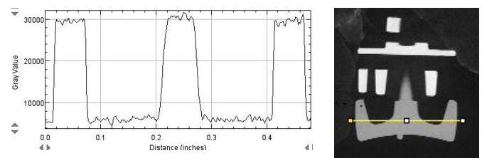
Fig. 5. Grey value profile (left) across the item at 0.11 mm from the bottom of the item (right).
