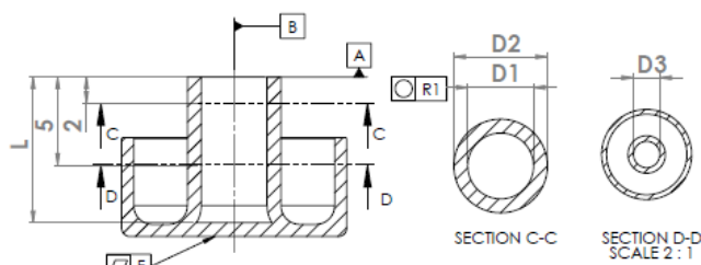
Fig. 2. The component and its datum system and measurands.
