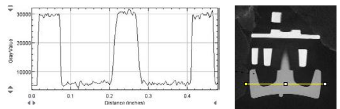
Fig. 5. Grey value profile (left) across the item at 0.11 mm from the bottom of the item (right).
