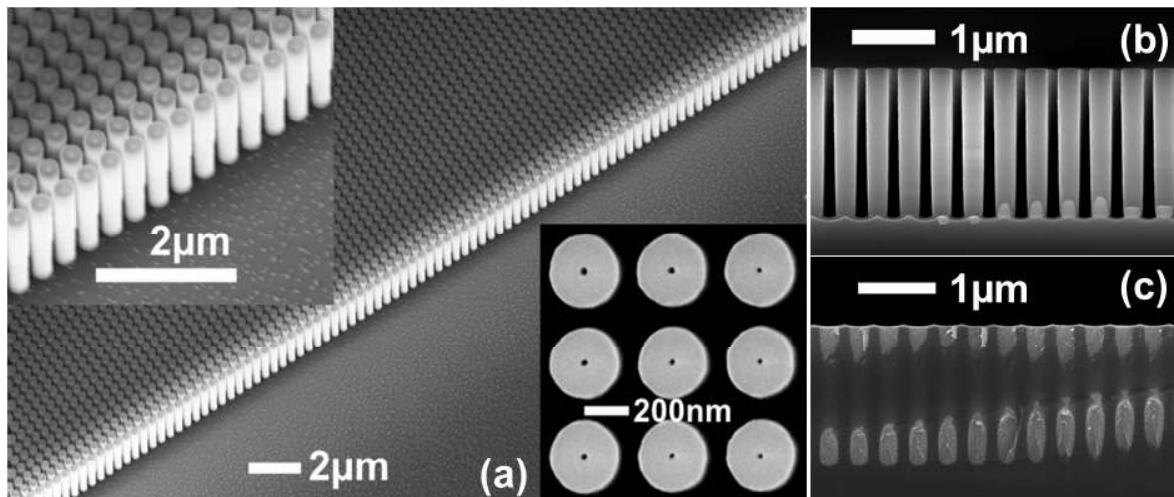
Fig. 1. (a) Scanning electron microscopy image of fabricated Al-doped ZnO (AZO) pillar structures in air surroundings with high aspect ratio. The insets show an enlarged view and a top view of the metamaterial. (b) Side view of AZO pillars in air and (c) AZO pillars in Si matrix.
