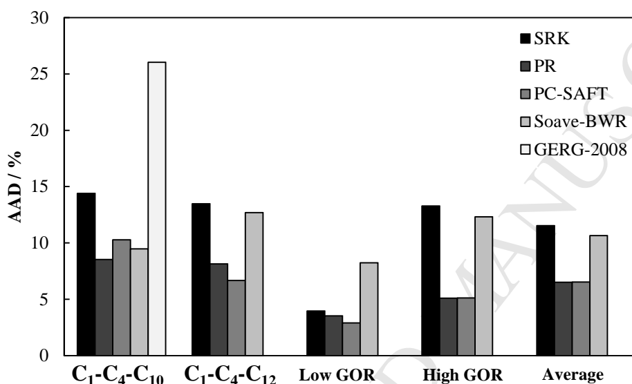
11 Figure 3. Absolute average deviations (AAD) obtained in the prediction of the saturation pressures 12 by different EoSs. 13 14
