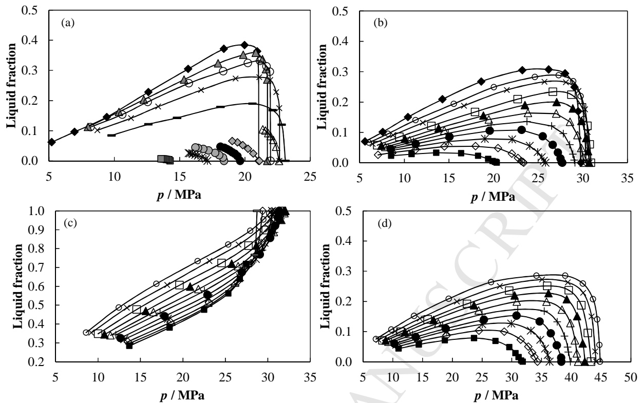
1 2 Figure 4. Liquid fraction upon expansion below the saturation pressure for the mixtures presented in 3 Table 3. (a) C 1 -C 4 -C 10 mixture, (b) C 1 -C 4 -C 12 mixture, (c) low GOR mixture and (d) high GOR 4 mixture. 283 K (◆), 293 K (▲), 298 K (○), 313 K (×), 333 K (□), 348 K (⇐), 353 K (▲), 373 K 5 (△), 393 K (+), 398 K (◆), 413 K (●), 423 K (●), 433 K (*), 448 K (■), 453 K (◇), 463 K (⇐), 6 473 K (■). The lines are drawn to guide the eyes.
