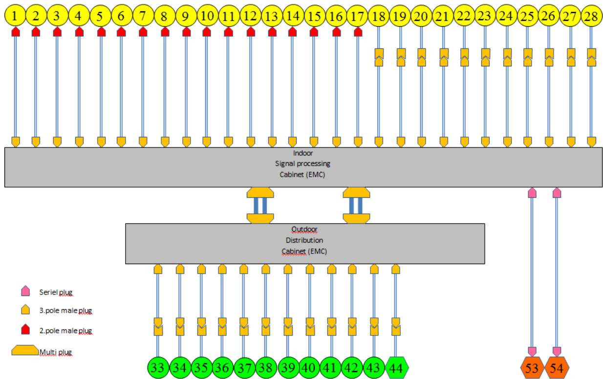
Figure 5. Connector types.
