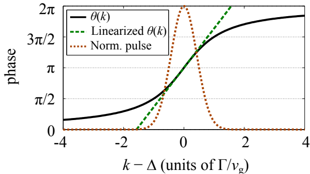
FIG. 2. Phase \theta(k) acquired by a single-photon wavepacket component with moment k propagating in a chiral waveguide scattering on a lossless resonant emitter (black solid line), together with a linear approximation, see Eq. (8) (green dashed line). By comparison, the spectrum of a resonant Gaussian wavepacket with spectral FWHM of \sigma = \Gamma/v_g is shown (orange dotted line) with a scaled intensity to match the plotting window.
