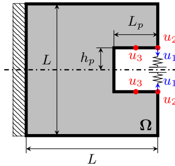
Figure 2. Design domain.
