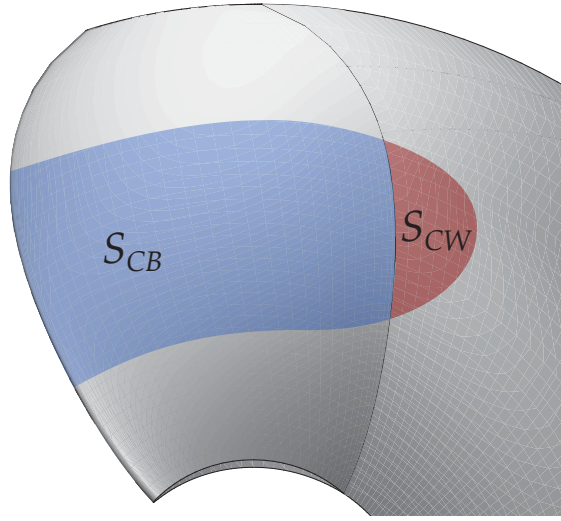
Figure 2.2: The cavitating parts of the blade and wake surfaces are subsets of the blade and wake surfaces, respectively: S_{CB} \subset S_B and S_{CW} \subset S_W
