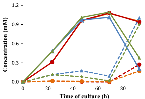
Fig. 5. Production of TS from cholesterol by a pseudo-resting-cell process. The strains Mycobacterium smegmatis MS6039-5941 (pHSDCT) and M. smegmatis MS6039-5941 (pHSDCL) were grown in minimal medium containing 18 mM glycerol (carbon and energy source) and 1.8 mM cholesterol (substrate) and, 1% glucose or glycerol was added at 69 h of culture. The following cultures were tested: MS6039-5941 (pHSDCT) with glucose (red); MS6039-5941 (pHSDCT) with glycerol (orange); MS6039-5941 (pHSDCL) with glucose (blue) and MS6039-5941 (pHSDCL) with glycerol (green). The AD concentration (continuous lines) and TS (dashed lines) are represented. A representative experiment is shown.
