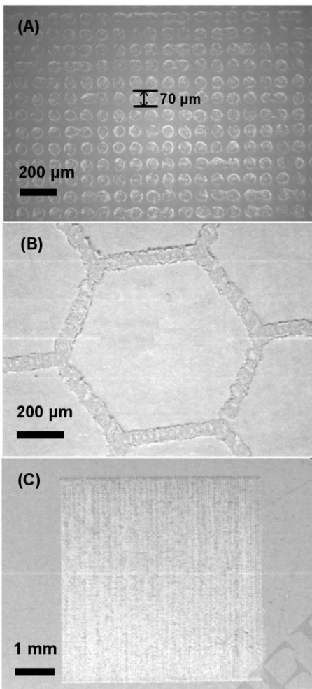
Figure 4: separated splats (A), honeycomb pattern (B) and continuous squared layer (C) all obtained using the ink with Z = 20 and by overprinting 10 times with a linear density of 500 dots per inch.
