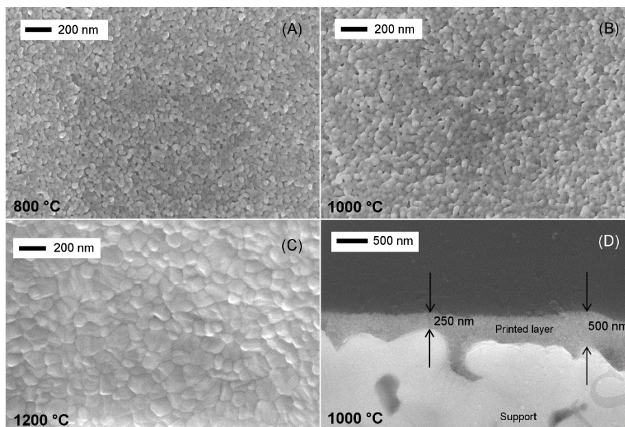
Figure 5: microstructure of YSZ nanoparticles after free sintering at 800 °C (A), 1000 °C (B), 1200 °C (C) , and cross-section of the printed film after sintering in constrained conditions at 1000 °C (D).
