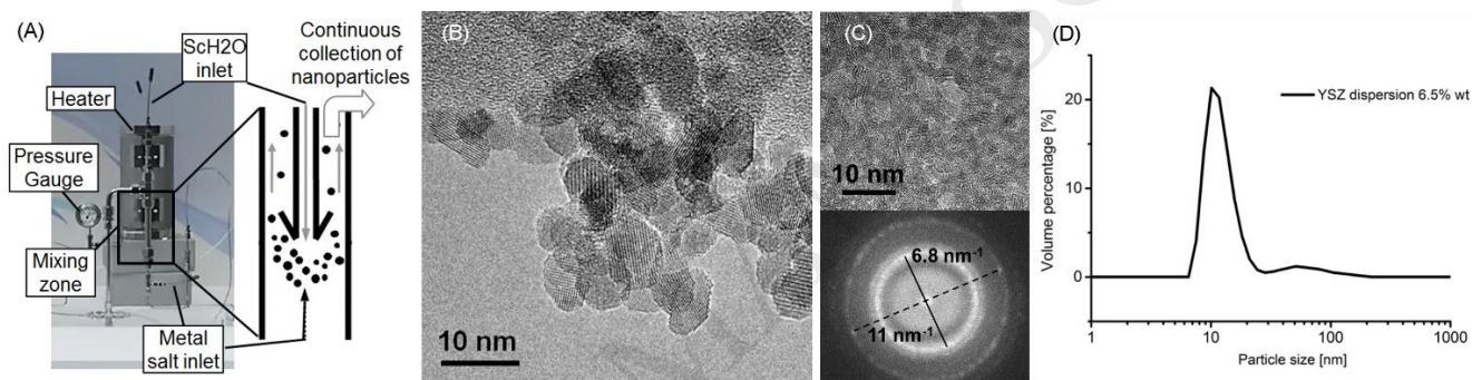
Figure 1: Sketch of the continuous hydrothermal reactor (Promethean Particles LTD.) with a magnified view of the mixing zone (A), TEM image of the YSZ nanoparticles produced at DTU Energy (B), and Fourier transform of a TEM image at low magnification with randomly distributed particles (C). Figure 1(C) reports the Fourier transform used for calculating the (220) and (111) planes distances. Figure 1(D) shows the DLS analysis of a synthesized YSZ dispersion.
