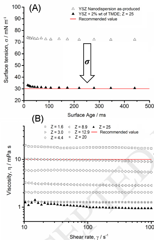
Figure 2: Rheological optimization of the YSZ nano-dispersions. Measurement of the surface tension before and after the addition of TMDE (A), viscosities at increasing shear rates and resulting Z values at 1000 \text{ s}^{-1} rate (B). The red line marks the surface tension and viscosity recommended by the printhead manufacturer for an optimal jetting.
