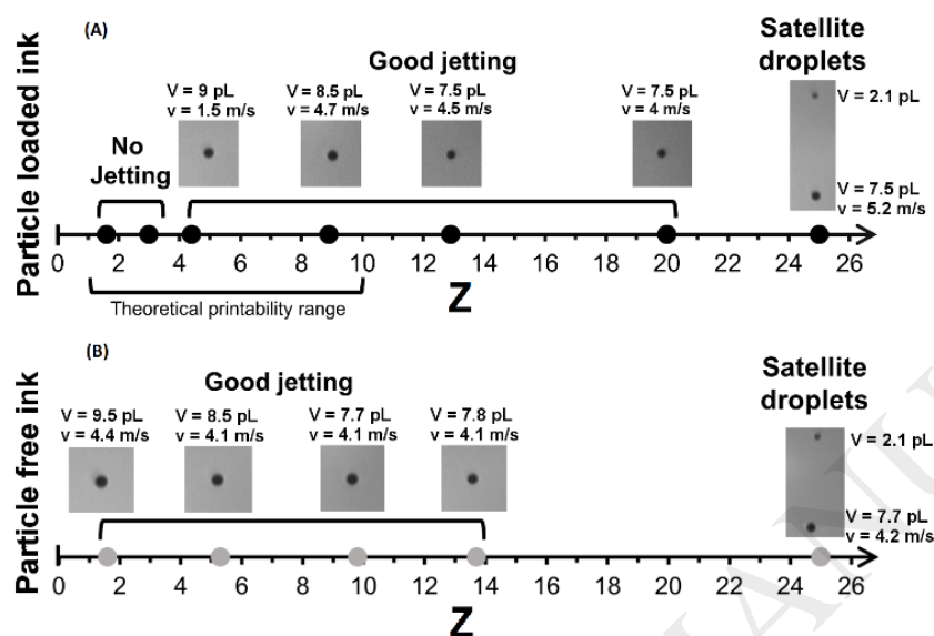
Figure 3: Jetting behavior of the formulated particle-loaded inks with different Z values (A). Jetting behavior of particle-free inks with similar Z values of the particle-loaded inks (B). Both (A) and (B) report a droplet picture, the droplet volume V and speed v obtained at each Z.
