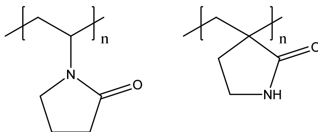
Figure 1. Poly( N -vinyl pyrrolidone) (left) and poly(3-methylene-2-pyrrolidone) (right).
