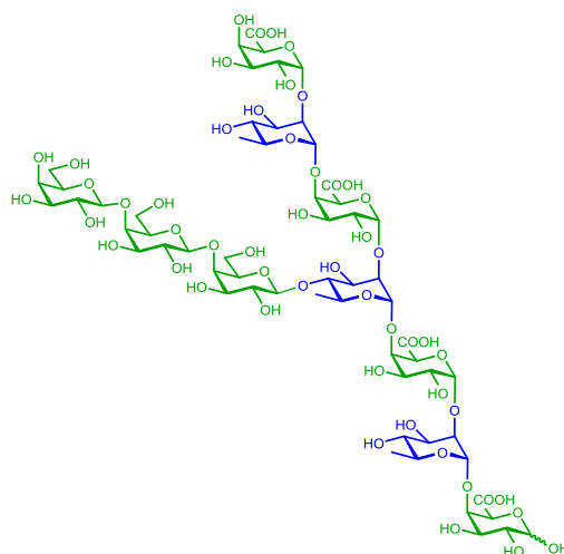
Figure 1. Branched-backbone synthetic target of the pectic RG-I polysaccharide.
