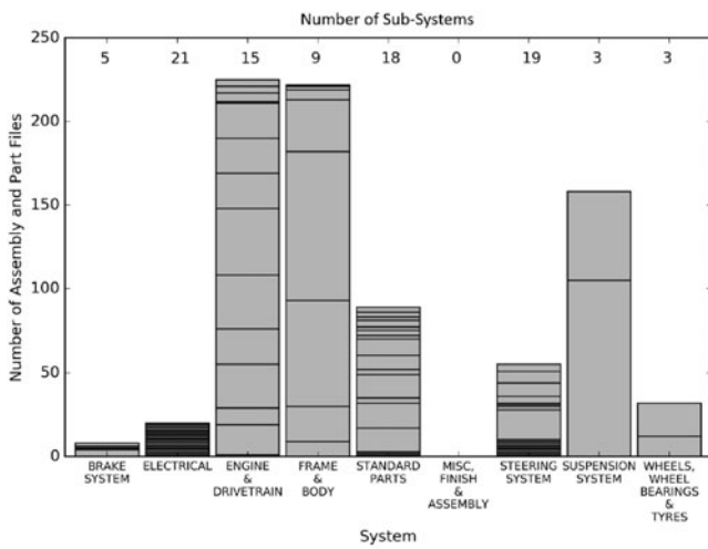
(a) Bath automated parts system subsystem structure
