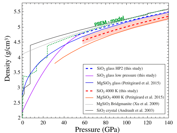
FIG. 3. \text{SiO}_2 density at room and high temperature. \text{SiO}_2 and \text{MgSiO}_3 [30] glass density at room temperature in dashed and continuous blue lines, respectively. In red, densities to lower-mantle temperatures of 4000 K. Density for \text{SiO}_2 crystals [38,39], bridgmanite [49], and the PREM model [50] are plotted for comparison. The red-shaded area represents the density at 4000 K with an error of 5% for possible uncertainties on the \text{SiO}_2 thermal expansion [47].
