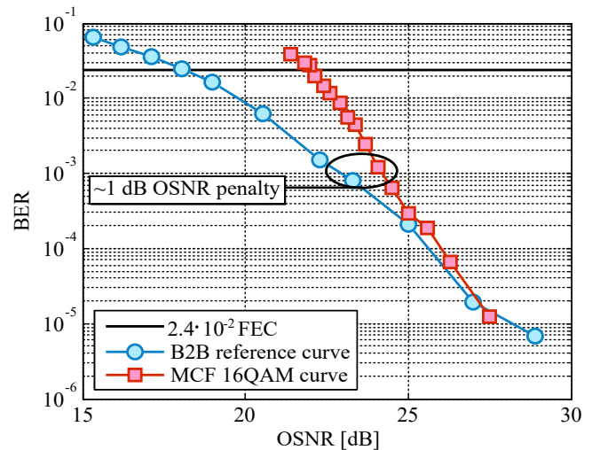
Fig. 11. BER vs. OSNR comparison between the optical B2B reference curve and the mapped points from Fig. 10
