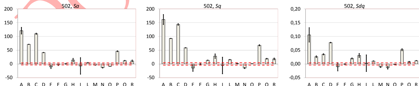
Figure 2. Left: S_a deviations for 502 type samples (random profile), expressed in nm. Centre: S_q deviations for 502 type samples, expressed in nm. Right: S_{dq} deviations for 502 type samples, dimensionless. Red dashed lines (- -) indicate the expanded uncertainty of AFM reference measurements. Bars on histograms indicate the expanded uncertainty of the measurements stated by the participants.
