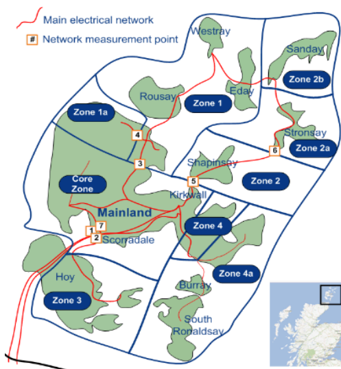
Figure 2 The main electrical grid in Orkney, showing the Active Network Management zones and main connection to the Scottish mainland.
