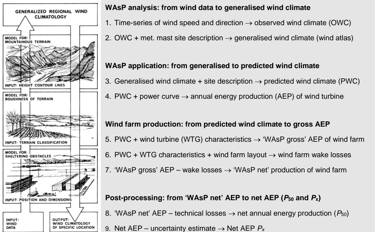
Figure 3. Wind atlas methodology of WAsP (Troen and Petersen, 1989). Meteorological models are used to calculate the generalised wind climatology from the measured data – the analysis part. In the reverse process – the application of wind atlas data – the wind climate at any specific site may be calculated from the generalised wind climatology.
