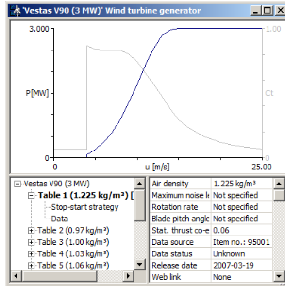
Figure 12. Power and thrust curves for a Vestas V90 3-MW wind turbine. Different tables (lower left) may correspond to different air densities or sound levels.
