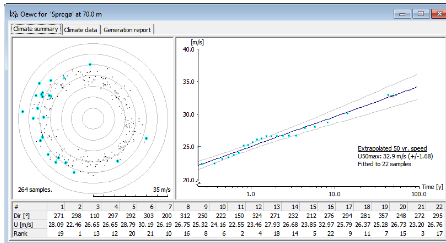
Figure 24. Sample observed extreme wind climate from Sprogø 1977-99; single events in a polar representation to the left and the extreme wind speed distribution with Gumbel fit to the right (data courtesy of Sund & Bælt). The 50-y extreme wind 70 m a.g.l. at this site is 32.9 \text{ ms}^{-1} , cf. Figure 7 for information on the mean wind climate.
