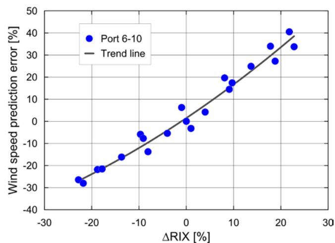
Figure 19. WASP wind speed prediction error in per cent as a function of the difference in ruggedness indices, \Delta RIX [%], between the predicted site and the predictor site. Data points represent cross-predictions between 5 masts in N Portugal.
