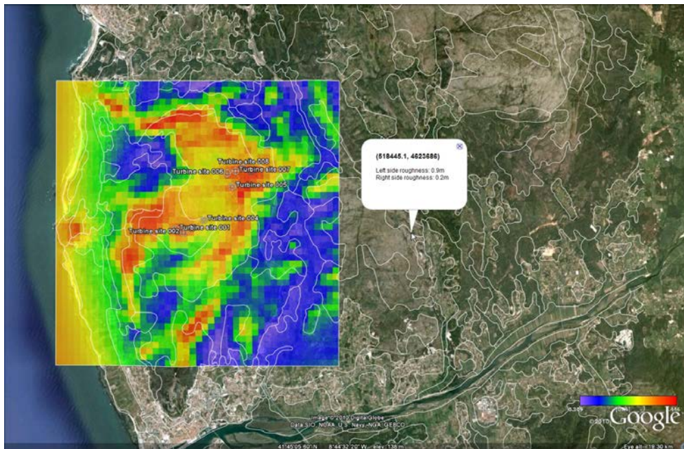
Figure 10. Land cover map for a site in Northern Portugal. The thin white lines show a land cover classification derived from the EU Corine 25-ha vector data set. A transformation table is needed for translating the land cover codes to roughness lengths.
