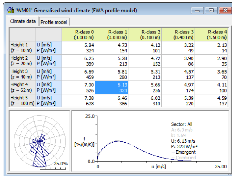
Figure 14. Sample wind atlas data set where the heights are adapted to site conditions. Data courtesy of the Wind Atlas for South Africa (WASA) project.
