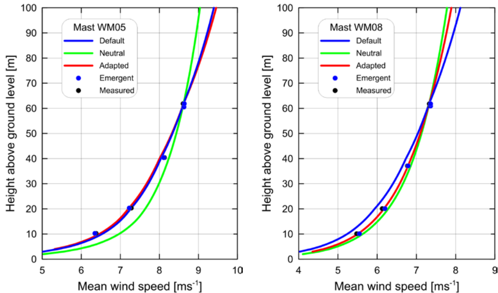
Figure 18. Measured and modelled vertical wind profiles at two sites in South Africa (data courtesy of the WASA project). The blue profile was modelled using the default setup of WASP 11; the green profile is a strictly neutral (logarithmic) wind profile, and the red profile has been adapted to the local conditions by changing the heat flux values in WASP slightly.
