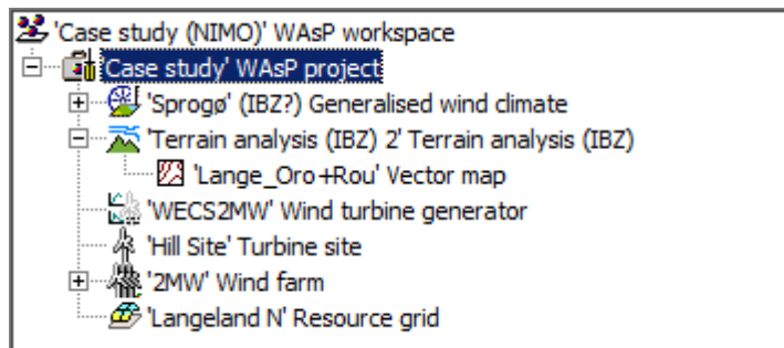
Figure 16. The generalised wind climate, a terrain analysis with vector map, and a wind turbine generator are inputs to the application; the turbine site, wind farm and resource grid contain the prediction results or outputs.
