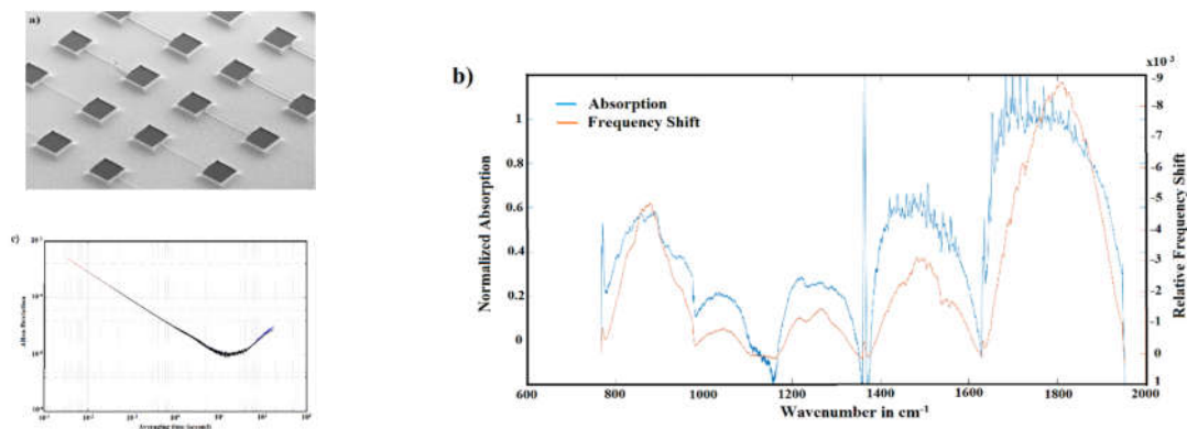
Figure 1: (a) SEM image, (b) IR absorption spectrum and (c) Allan Deviation plot of 400x15 \mu\text{m} pyrolytic carbon string resonator.
