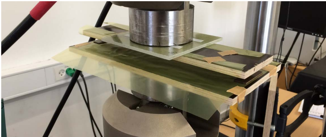
Figure 1: Test setup for the SF experiments.
