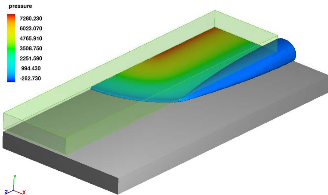
Figure 4: Prediction by the 3-D numerical model.
