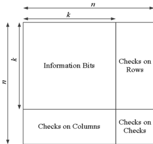
Fig. 1 Frame with product code structure.
