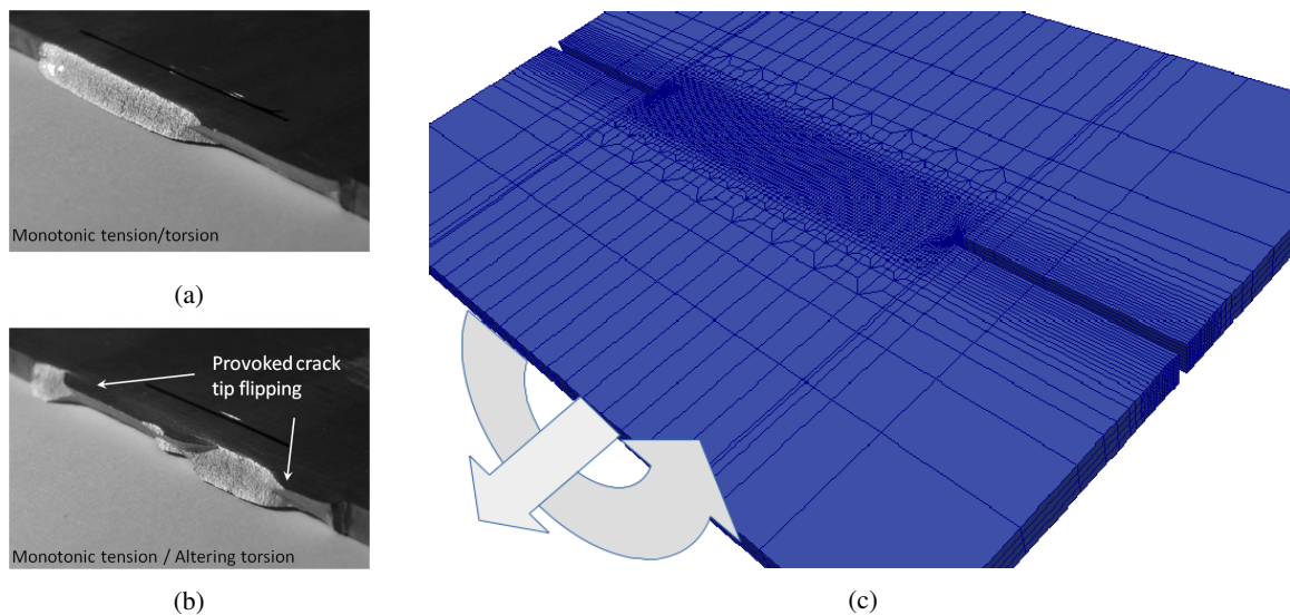
Figure 1: Axial displacement 1 mm/min. (a) 1^\circ/\text{min} CW twist, (b) 1^\circ/\text{min} CW twist followed by 3^\circ/\text{min} CCW twist, (c) Mesh for numerical analysis at initial condition indicating axial displacement and clock-wise (CW) twist of lower part.
