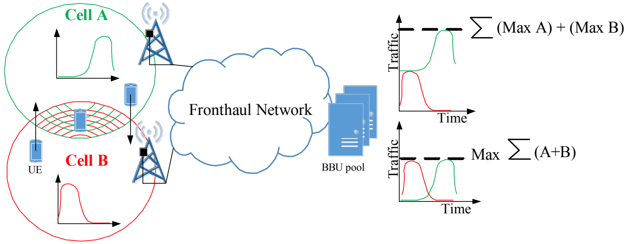
Fig. 1: C-RAN with interference between cells and shared processing in the BBU pool
