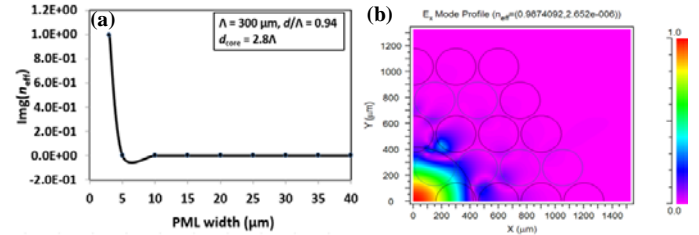
Fig. 4. (a) Variation of the imaginary part of the effective index as a function of PML width. (b) 2-D mode field profile (x component of the E -field) of the fundamental mode; only 1 st quadrant is plotted owing to an obvious symmetry in the structure.
