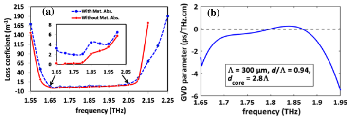
Fig.5. (a) Variation of transmission loss [with (blue dashed) and without (red solid) material absorption] and (b) GVD parameter as a function of THz frequency for the fundamental mode of the proposed HC-mPOF. The inset in ‘a’ shows an expanded view of the two loss spectra.
