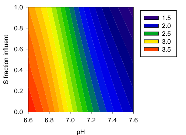
Figure 1: Influence of changing the pH vs. S (sulfate + sulfide) fraction in the influent on the reactor performance index (RPI) in M€year. Point A = default conditions; point B = influent S is removed; point C = pH decrease to 6.8.
