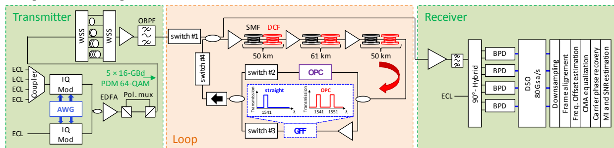
Fig. 1. (a) Experimental setup for the dispersion-compensated transmission with OPC: inset shows the transmission profiles for the GFF opening only the signal band and both signal and idler band for straight and OPC-based transmissions, respectively.
