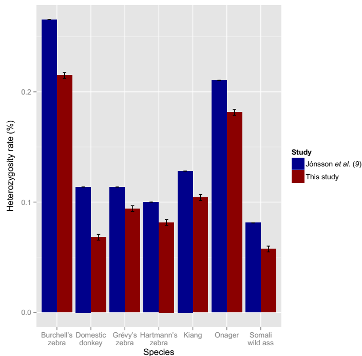
Fig. 2. Heterozygosity rates for various equine species. The heterozygosity estimates were computed using the same data aligned both to the horse genome (EquCab2.0) from a previous study and to the donkey reference presented in this study.
