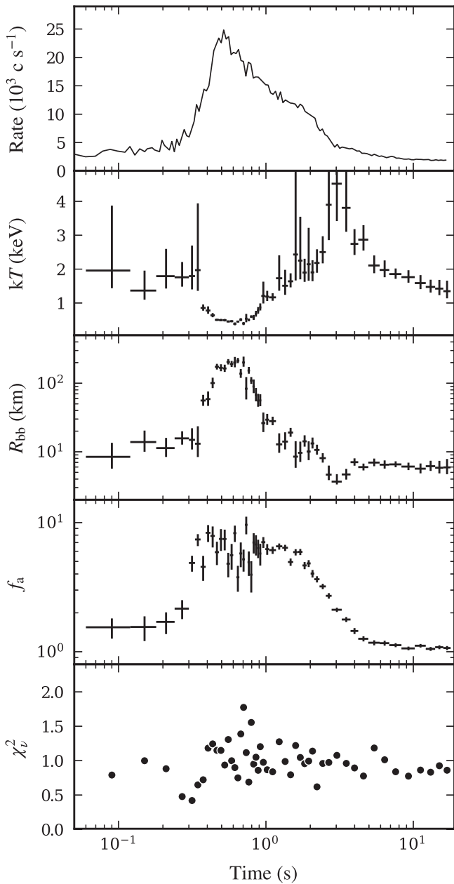
Figure 3. Results of time-resolved spectroscopy. The top panel shows the count rate, the bottom panel shows the goodness of fit \chi^2_v , and the other panels show the best-fitting values with 1\sigma errors for the blackbody temperature kT , radius of the emitting area R_{\text{bb}} (assuming a distance of 8.4 kpc), and scaling factor for the persistent Comptonization flux f_a .
