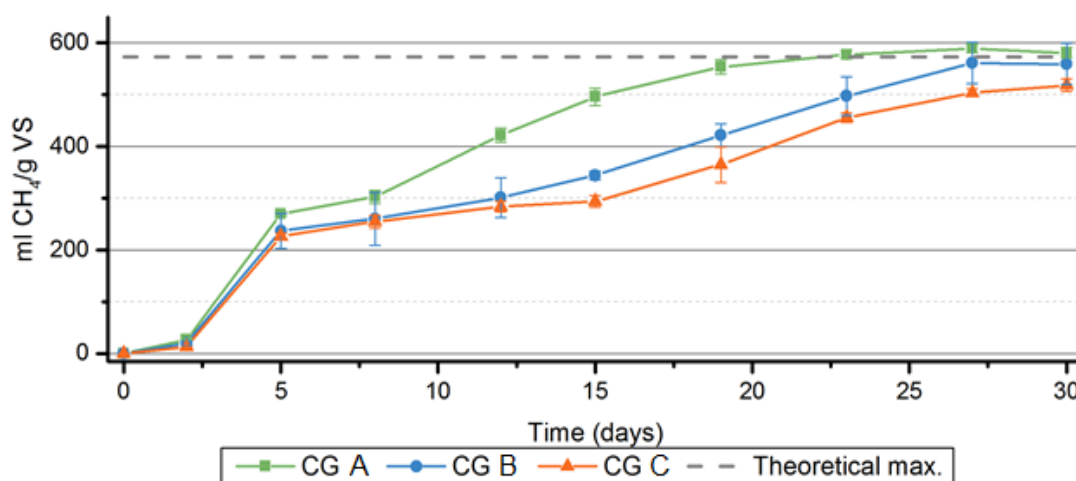
Figure 1. Cumulative CH 4 yields of BMPs of CG at different organic loadings. CG A, B and C correspond to I:S ratio on a VS basis of 4:1, 2:1 and 1:1 respectively.
