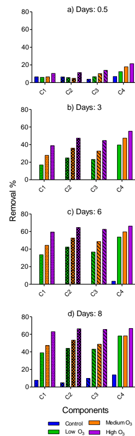
Figure 1: Effect of ozone on FDOM over time.
