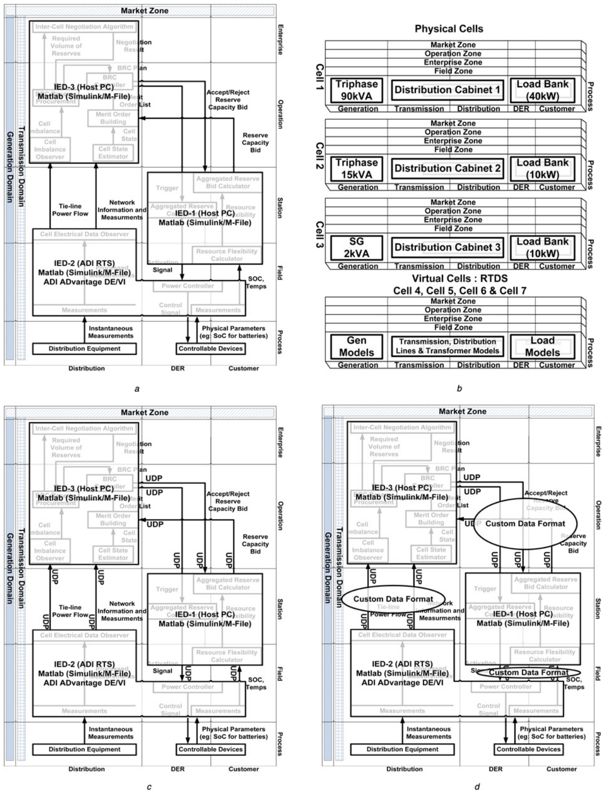
Fig. 4 SGAM layers
