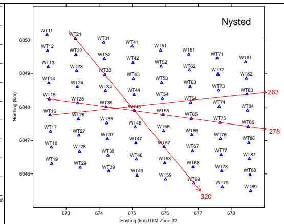
Figure 3. The Nysted wind farm layout with the selected wind directions.
