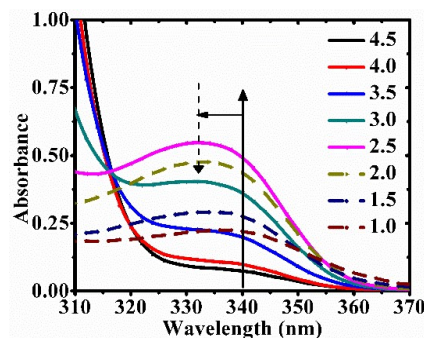
Figure 2. Degradation of NADH at pH 1.0 to 4.5. General conditions: NADH (1.4 mg, 2 μmol); phosphate buffer (2 mL); 3 h; 37 °C.
